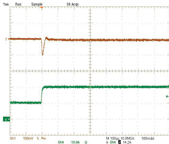
Step Load Transient Response (Vin=12V, Vout=1.2V, Cloud=188μF, Iout=10A to 20A) Trace 1=Vout, 100 mV/div(AC), Trace 4=Iout, 10A/div.
