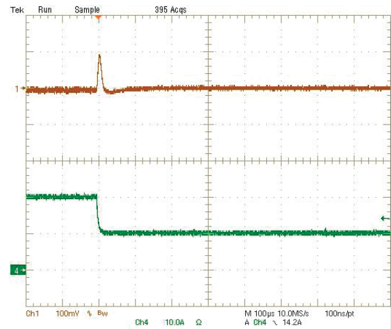
Step Load Transient Response (Vin=12V, Vout=2.5V, Cloud=188μF, Iout=20A to 10A) Trace 1=Vout, 100 mV/div(AC), Trace 4=Iout, 10A/div.
