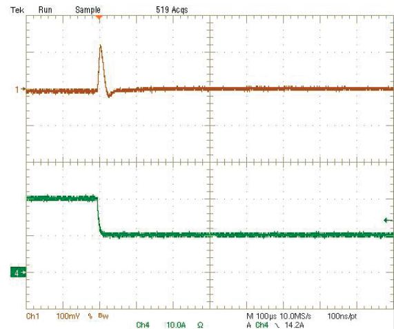
Step Load Transient Response (Vin=12V, Vout=1.2V, Cloud=188μF, Iout=20A to 10A) Trace 1=Vout, 100 mV/div(AC), Trace 4=Iout, 10A/div.
